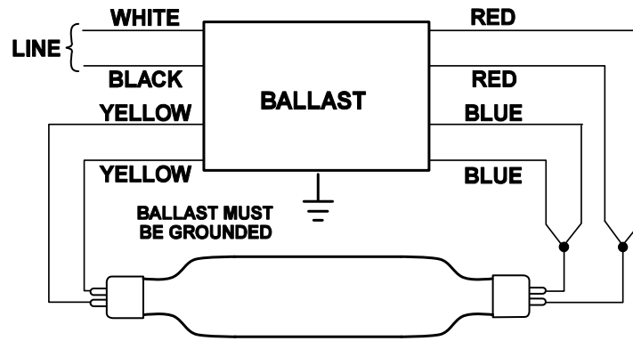
Figure 2 – Wiring Diagram
