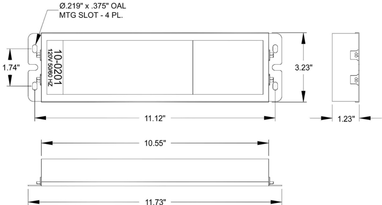
Figure 1- Dimensional Data
