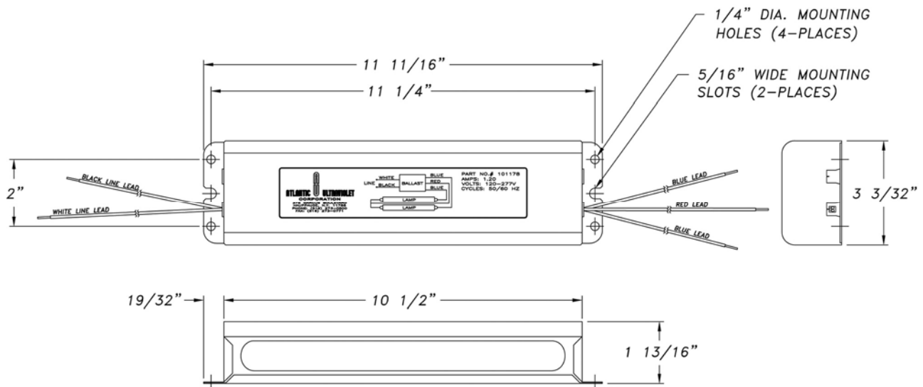
Figure 1- Dimensional Data
