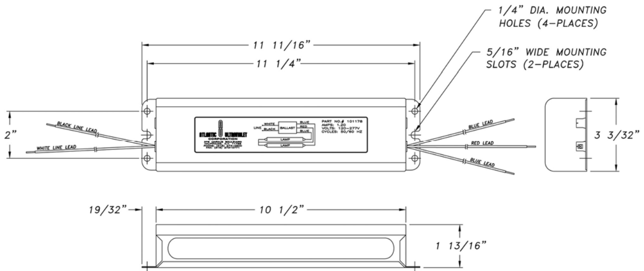
Figure 1- Dimensional Data
