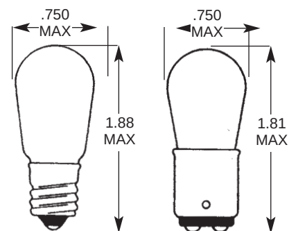
CANDELABRA SCREW BASE
