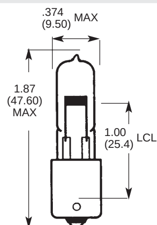
S.C. BAYONET BASE
