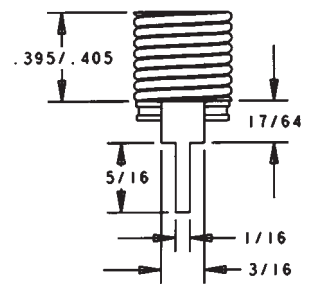
STANDARD MOUNT
