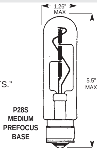
P28S MEDIUM PREFOCUS BASE
