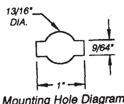
Mounting Hole Diagram
