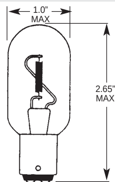
D.C. BAYONET BASE
