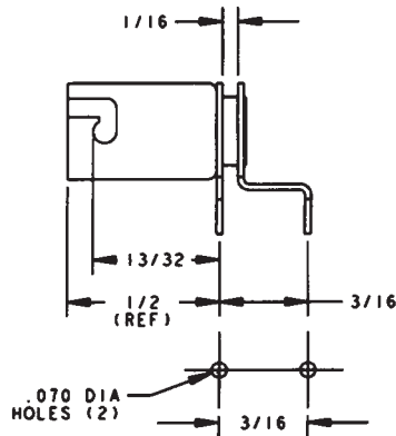
RT. ANGLE MOUNT
