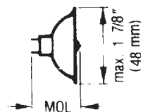
G-4 2-PIN BASE
