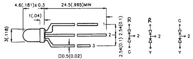
COMMON CATHODE (2)
