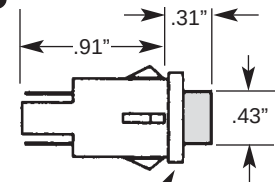
.63" SQUARE STAINLESS STEEL BEZEL
