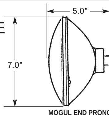
MOGUL END PRONG
