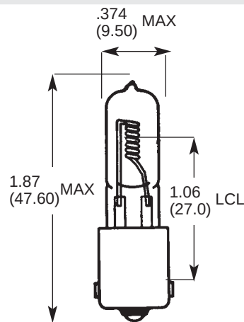
S.C. BAYONET BASE
