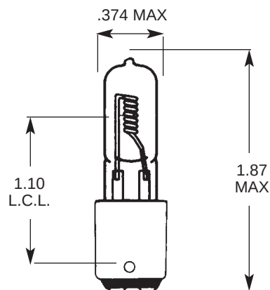
D.C. BAYONET BASE
