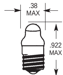
GTL-3 LENS END
