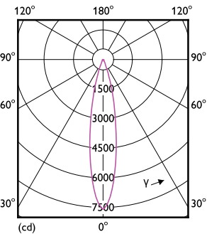
Light Distribution Diagram - 14PAR38/EXPERTCOLOR RETAIL/F25/930/P/D
