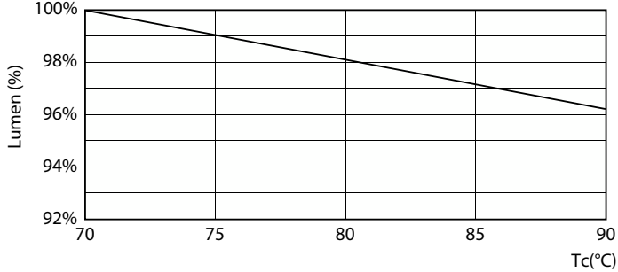
Lumen Maintenance Diagram - 15.5T8/COR/48-835/MF21/G/BAA 25/1
