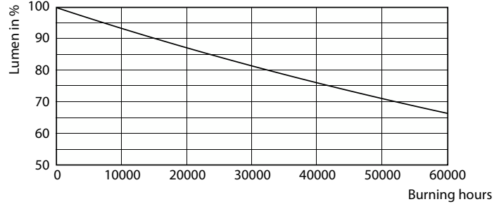
Lumen Maintenance Diagram - 15.5T8/COR/48-835/MF21/G/BAA 25/1
