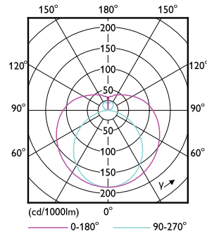
Light Distribution Diagram - 15.5T8/COR/48-835/MF21/G/BAA 25/1
