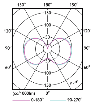
Light Distribution Diagram - 150CC/LED/850/LS EX39 G2 BB 277-480V 3/1
