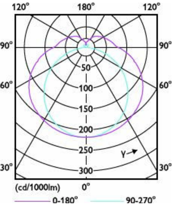
Light Distribution Diagram - 16.5PL-L/COR/22-830/IF22/P/4P/DIM 10/1
