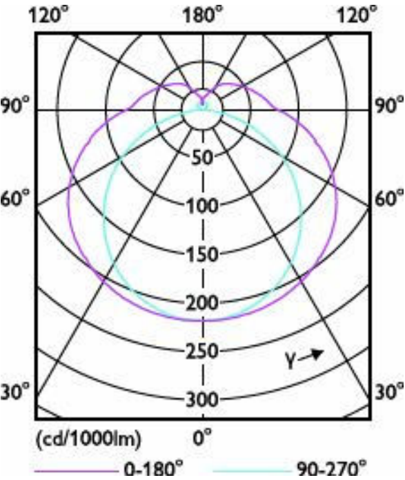
Light Distribution Diagram - 16.5PL-L/COR/22-835/IF22/P/4P/DIM 10/1
