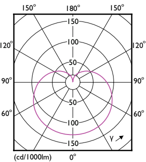
Light Distribution Diagram - 16.6A19/LED/930/FR/P/E26/ND/T20 6/1FB
