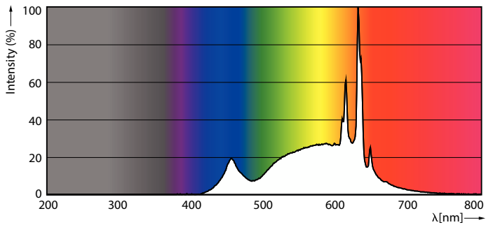
Spectral Power Distribution Colour - 16.6A19/LED/930/FR/P/E26/ND/T20 6/1FB
