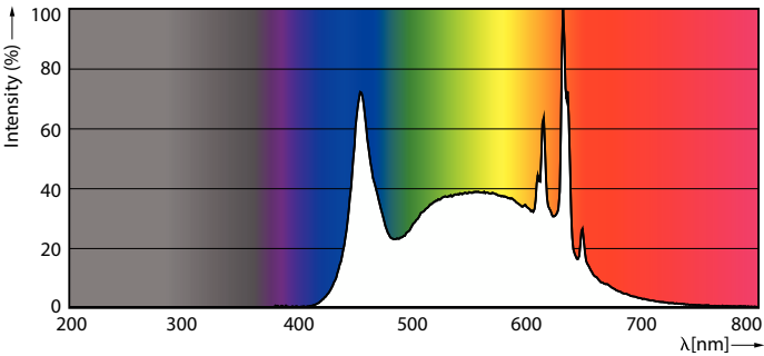
Spectral Power Distribution Colour - 16.6A19/LED/950/FR/P/E26/ND/T20 6/1FB
