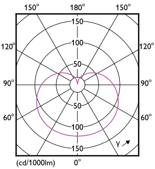
LEDbulb A19 16W E26 1600lm 940 FR
