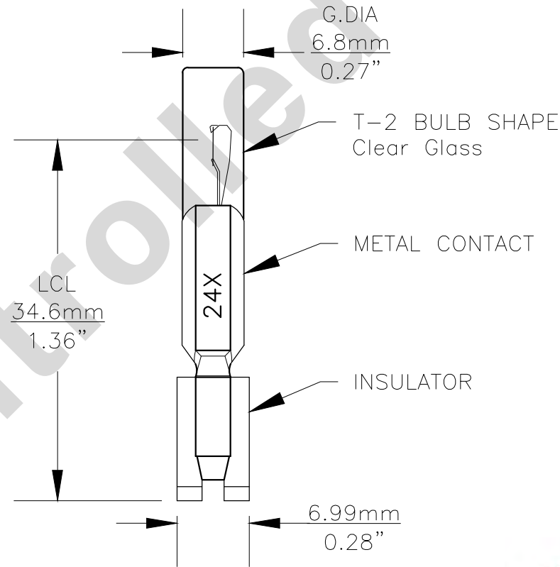
90° VIEW
