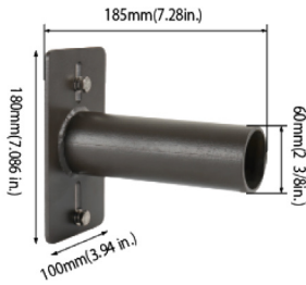
Inner Diameter 54mm SQ-SP-D
