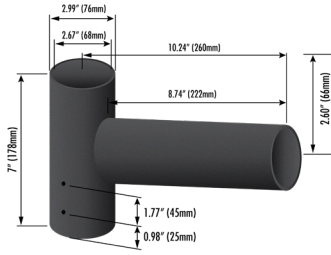
Side Inner Diameter : 56mm Lower Inner Diameter : 64mm R60-SP1-D
