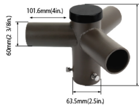
Side Inner Diameter : 56mm Lower Inner Diameter : 64mm R60-SP3-120-D
