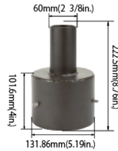
Top Inner Diameter : 54mm Lower Inner Diameter : 132mm 5SQR-SP-D
