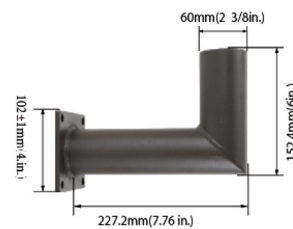
Inner Diameter 54mm WM-SP-D
