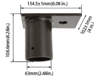
Inner Diameter 64mm SP-TR-D
