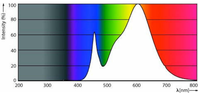
Spectral Power Distribution Colour - 54GC/MAS/840 EX39 BB 6/1
