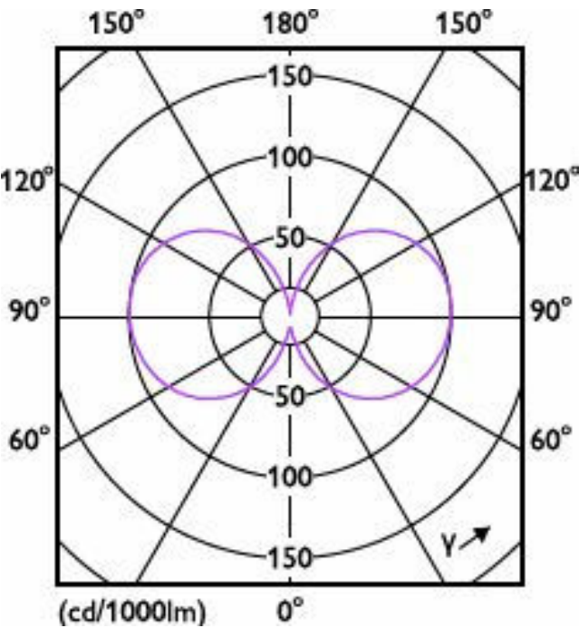
Light Distribution Diagram - 54GC/MAS/840 EX39 BB 6/1
