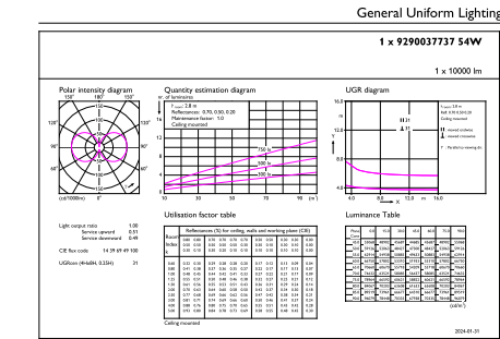
Light Distribution Diagram - 54GC/MAS/840 EX39 BB 6/1
