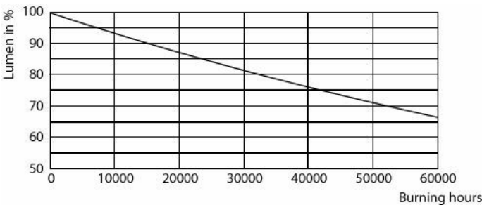
Lumen Maintenance Diagram - 54GC/MAS/840 EX39 BB 6/1
