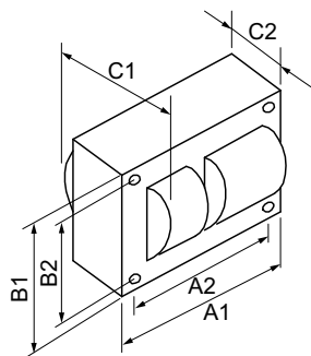
HPS BAL 150W S55 480V KIT
