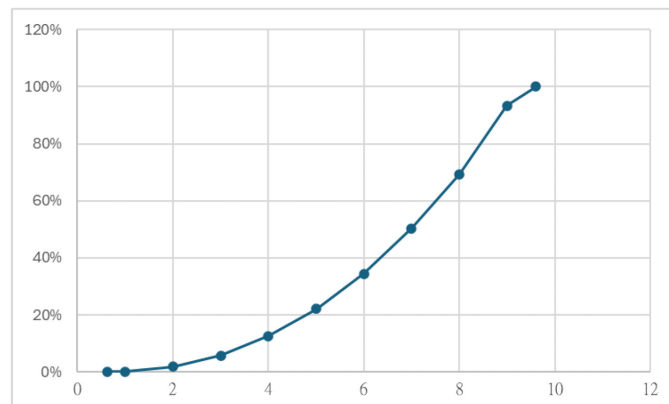
LOGARITHMIC DIMMING
