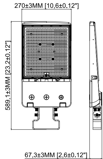
Trunnion
