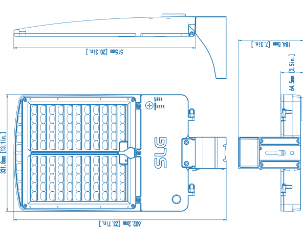
ALF LS500 and LS600 - with Pole Mount
