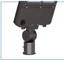
Slipfitter Mount An optional cast aluminum mast arm adapter secures fixture head to nominal 2-3/8\"/>
