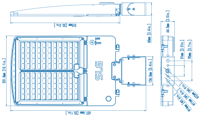
ALF LS500 and LS600 - with Trunnion Mount
