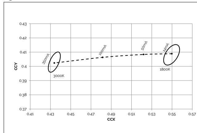
Figure 12: Color shift vs. Forward Current 3000K - 1800K
