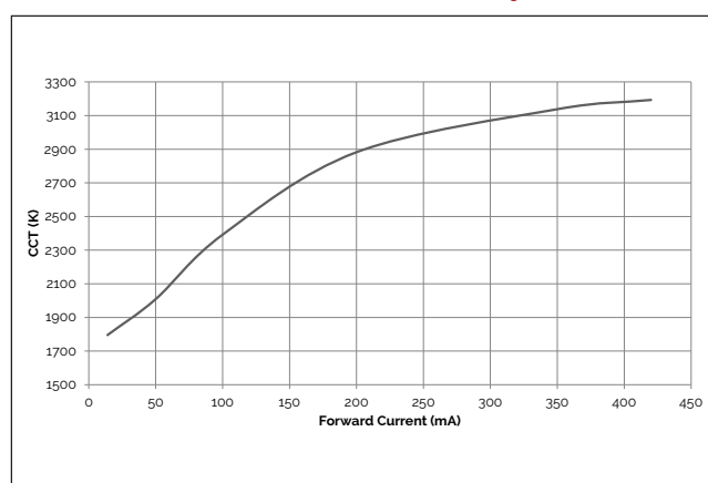
Figure 6: 6W CCT vs. Forward Current, T_c = 25^\circ\text{C}
