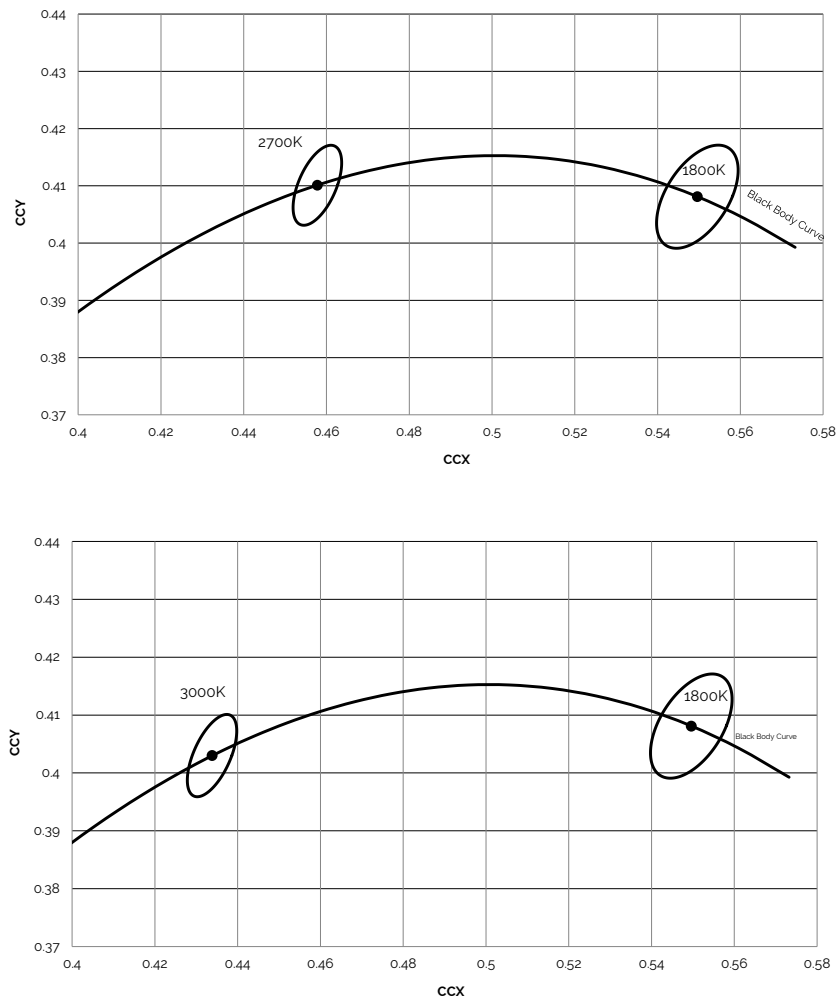
Figure 19: Graph of Warm White Test Bins in xy Color Space
