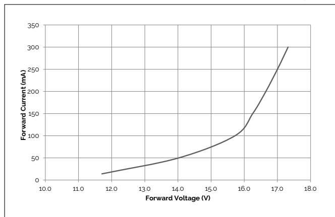
Figure 1: 4W Forward Voltage vs. Forward Current, T_c = 25^\circ\text{C}
