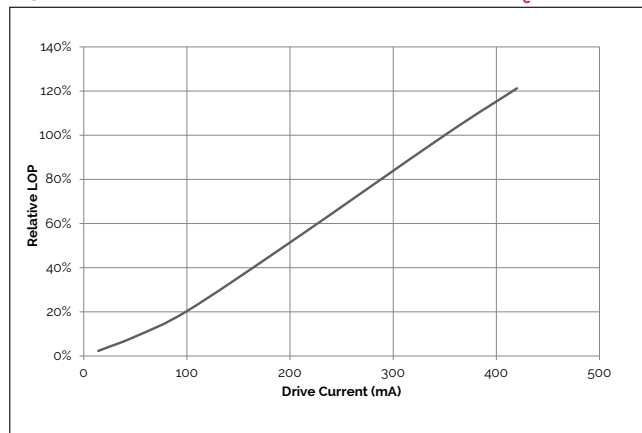
Figure 9: 6W Relative LOP vs. Drive Current, T_c = 25^\circ\text{C}
