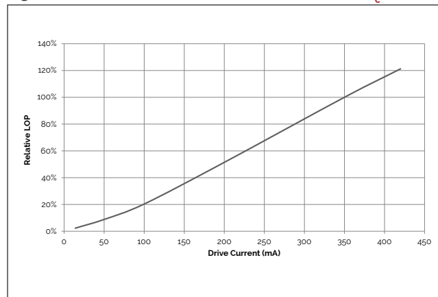
Figure 10: 12W Relative LOP vs. Drive Current, T_c = 25^\circ\text{C}
