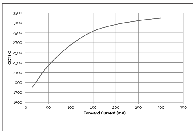
Figure 5: 4W CCT vs. Forward Current, T_c = 25^\circ\text{C}
