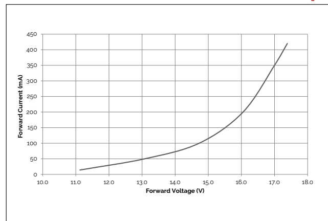
Figure 2: 6W Forward Voltage vs. Forward Current, T_c = 25^\circ\text{C}
