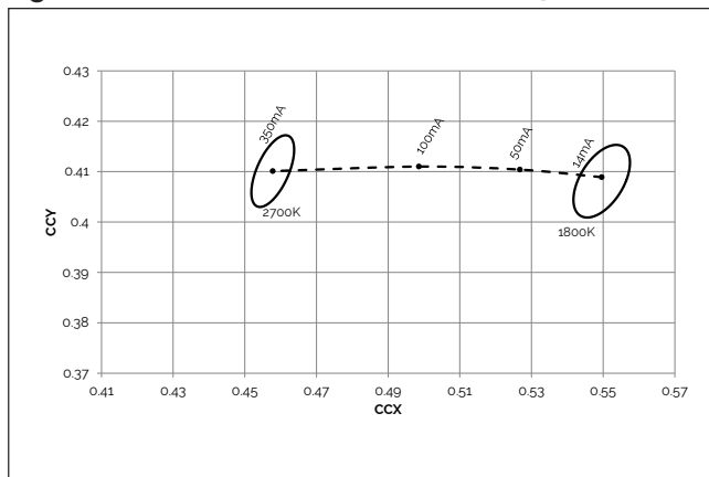
Figure 11: Color shift vs. Forward Current 2700K - 1800K
