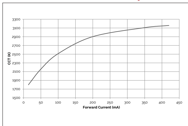
Figure 7: 12W CCT vs. Forward Current, T_c = 25^\circ\text{C}
