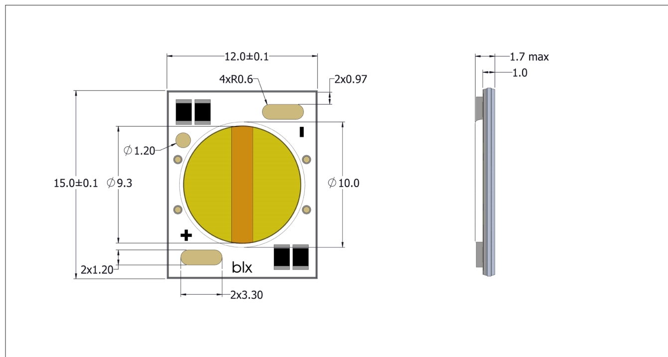
Figure 18: Drawings for Vesta Dim-To-Warm 9mm Array
