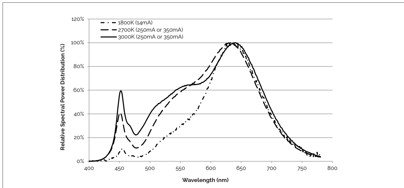
Figure 17: Typical Color Spectrum
