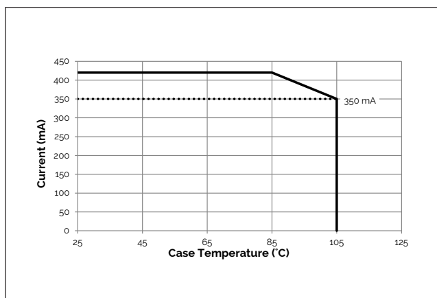
Figure 14: Derating Curve 6W, 12W
