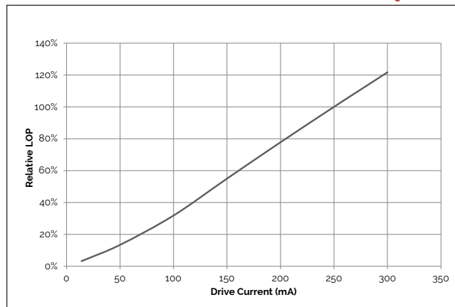
Figure 8: 4W Relative LOP vs. Drive Current, T_c = 25^\circ\text{C}
