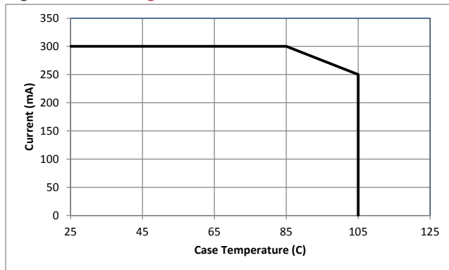
Figure 13: Derating Curve 4W
