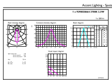
LEDspot Classic MR11 36D 2700K
