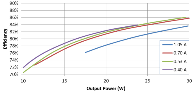
Efficiency Vs. Output Power, 277V In
