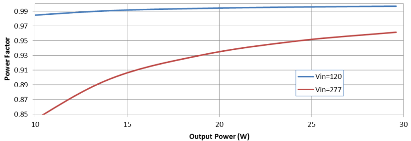
PF vs Output Power
