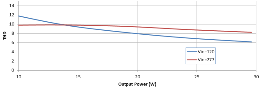
THD vs Output Power
