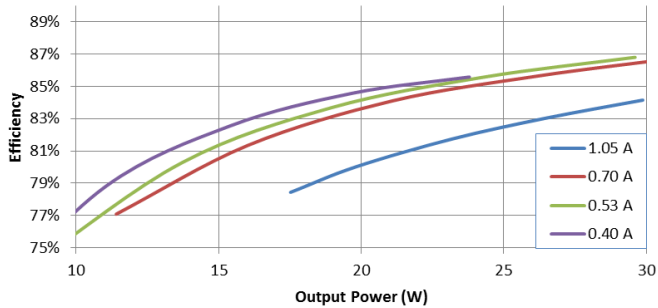
Efficiency Vs. Output Power, 120V In
