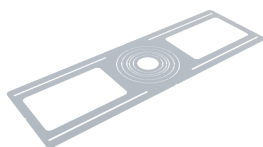
DR-MOUNTING-PLATE Round cut out 2.1"3" 3.75"4.25" 5.25"6.25". Work with 2/3/4/6 round downlight.
