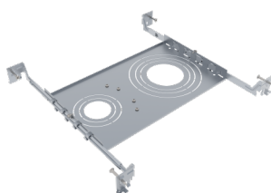
DRR-UNV-HOUSING Integrated with T-bar, Dual rows round, big one cutout is: 3.2" 4.3" 5.2" 6.3", work with 3/4/5/6 inch round downlight, small one cut out is 2.1" 2.8" 3.7" work with 2/3 inch round downlight.
