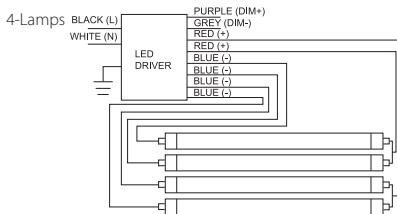
fig. 5 Retrofit with Four Lamps
