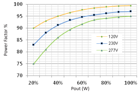
PF vs. Pout at 80°C case
