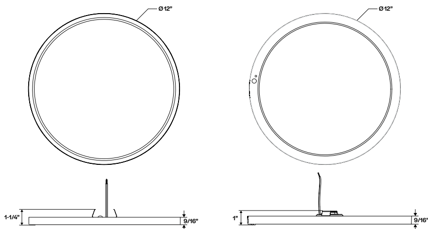
DSK-12-CS-120V
