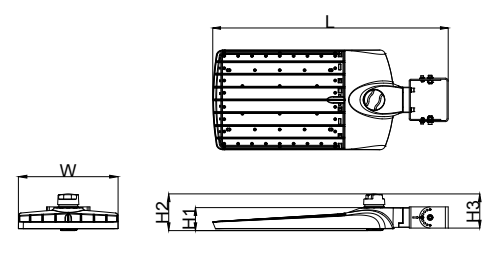
Yoke Mount (YK)
