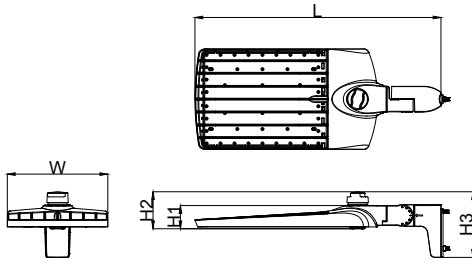
Adjustable Round / Square Mount (ASRP)
