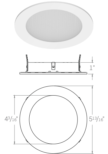
ED5-RFWL ROUND WET LOCATION
