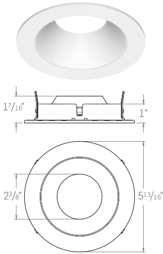
ED5-RFST ROUND FIXED STANDARD TRIM
