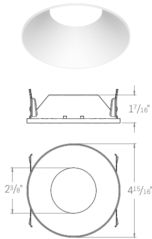
ED5-RFTL ROUND FIXED TRIMLESS
