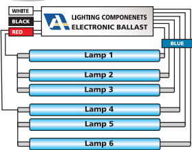
WIRING DIAGRAM 4
