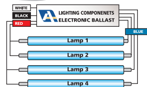
WIRING DIAGRAM 5
