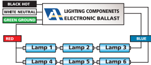
WIRING DIAGRAM 8
