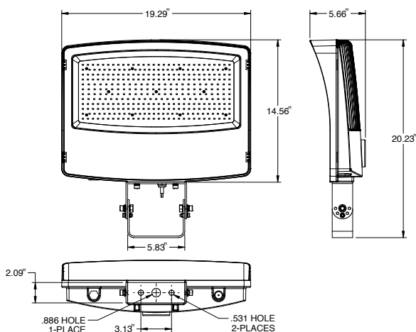
EFP1 200W & 320W- size 3 (Trunnion)
