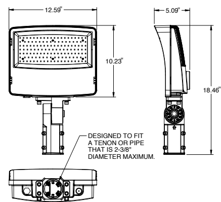
EFP1 120W- size 2 (knuckle)
