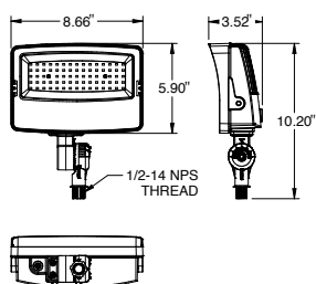
EFP1 60W Size 1
