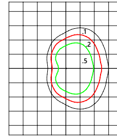
ERL1 Type IV Short Visual Comfort Lens 14601 Lumens 4000K ERL1_16M740___IES
