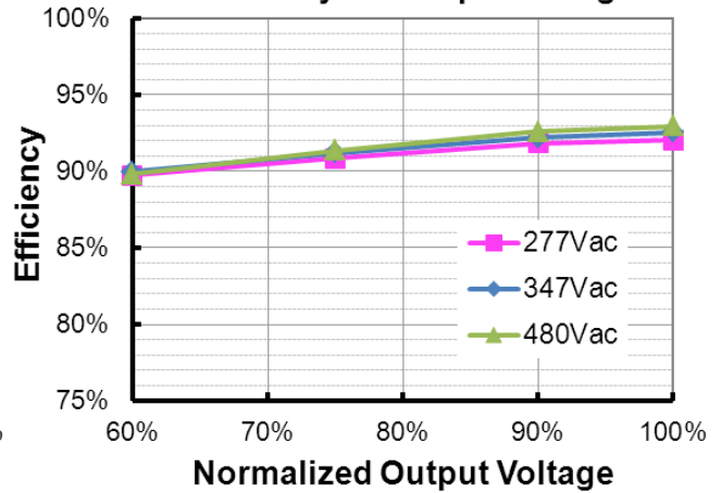
ESD-480S560DT (I o =5600mA) Efficiency vs. Output Voltage
