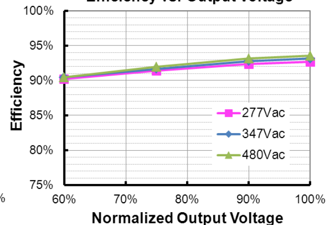
ESD-480S420DT (I o =4200mA) Efficiency vs. Output Voltage
