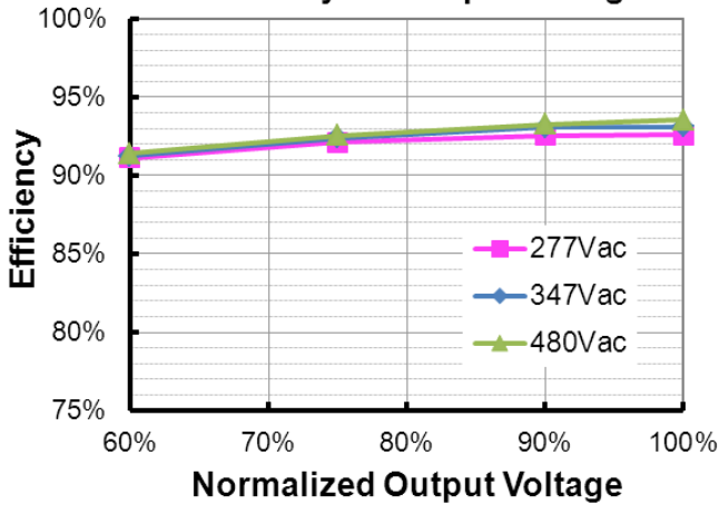
ESD-480S560DT (I o =4350mA) Efficiency vs. Output Voltage
