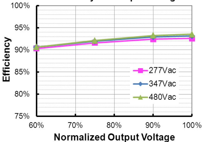
ESD-480S10ADT (I o =7500mA) Efficiency vs. Output Voltage
