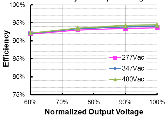
ESD-480S420DT (I o =3150mA) Efficiency vs. Output Voltage
