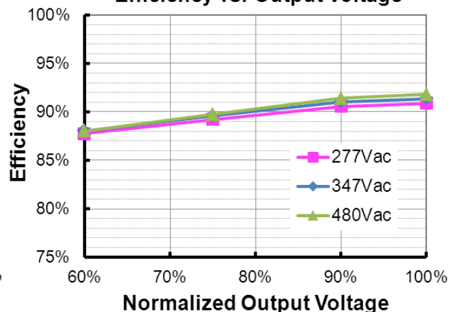
ESD-480S10ADT (I o =10000mA) Efficiency vs. Output Voltage
