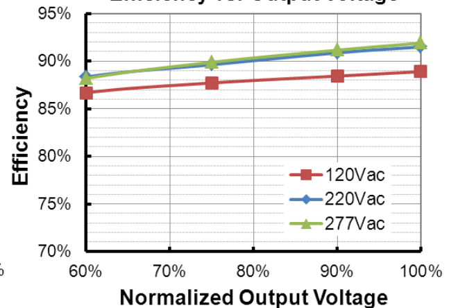
EUG-240S210DT( I_o=2100\text{mA} ) Efficiency vs. Output Voltage
