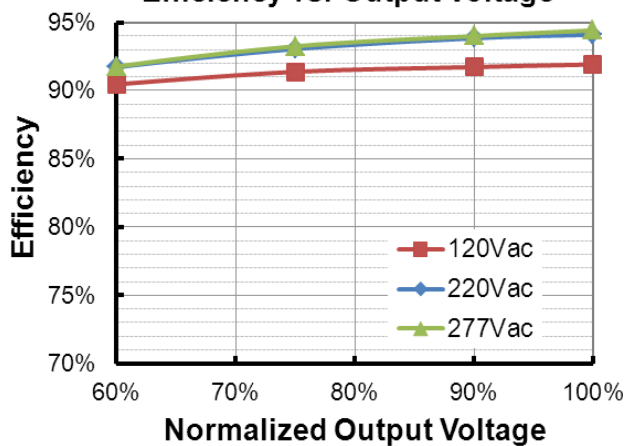
EUG-240S210DT( I_o=1400\text{mA} ) Efficiency vs. Output Voltage
