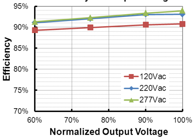
EUG-240S210DT( I_o=1400\text{mA} ) Efficiency vs. Output Voltage
