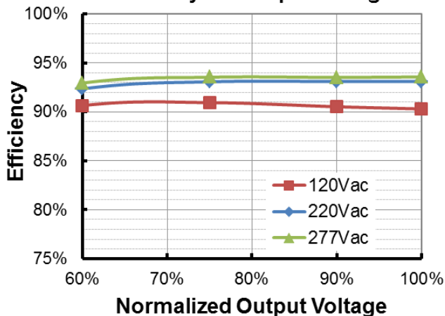
EUM-200S150Dx(I o =1050mA) Efficiency vs. Output Voltage
