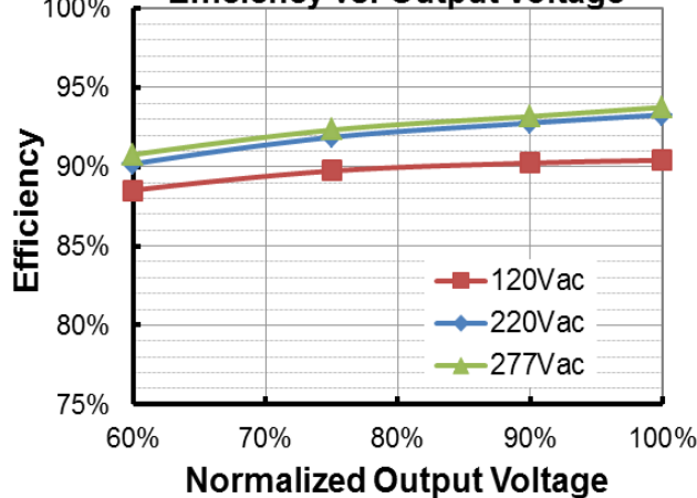
EUM-200S280Dx(I o =2800mA) Efficiency vs. Output Voltage
