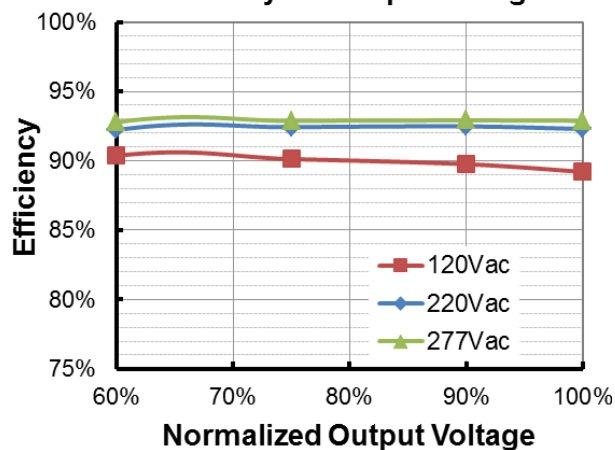
EUM-200S280Dx(I o =1800mA) Efficiency vs. Output Voltage
