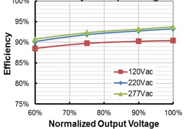
EUM-200S150Dx(I o =1500mA) Efficiency vs. Output Voltage
