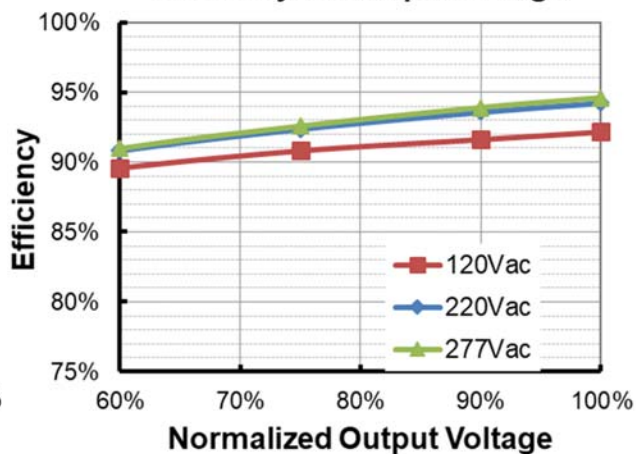
EUM-320S250Dx(Io=2500mA) Efficiency vs. Output Voltage
