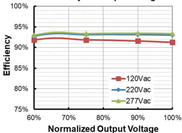
EUM-320S500Dx(Io=2850mA) Efficiency vs. Output Voltage
