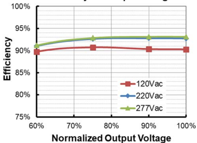
EUM-320S760Dx(Io=5350mA) Efficiency vs. Output Voltage
