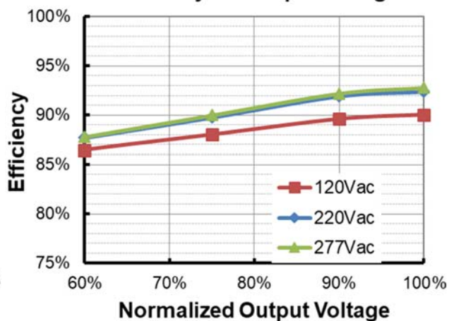
EUM-320S760Dx(Io=7600mA) Efficiency vs. Output Voltage
