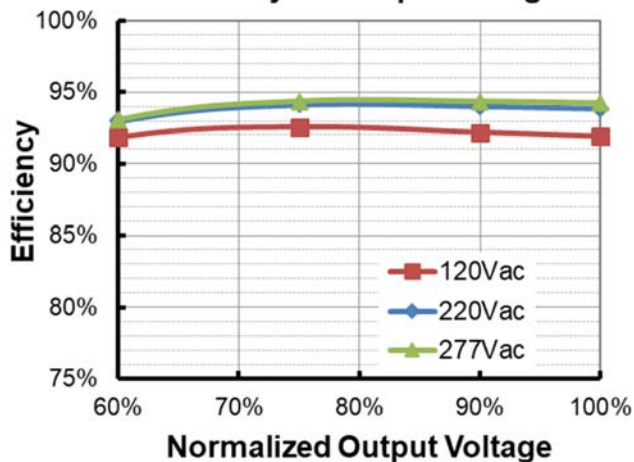
EUM-320S250Dx(Io=1750mA) Efficiency vs. Output Voltage
