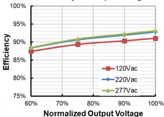
EUM-320S500Dx(Io=5000mA) Efficiency vs. Output Voltage
