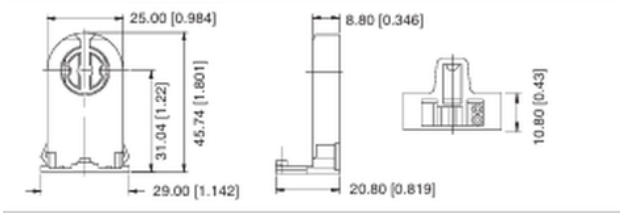
FL205-SN Flexible Shoulder, Shunted T-8 Only, Locating Nib
