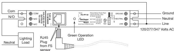
Fig 2: FS-PP v2 direct wiring to lighting load
