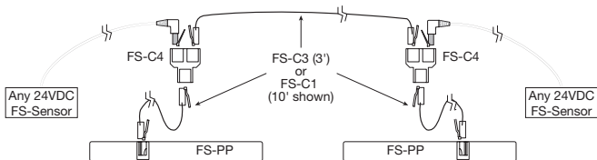
Fig 8: Two sensors controlling two Power Packs
