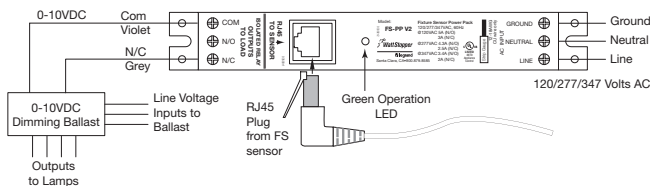
Fig 3: FS-PP v2 wiring to 0-10V dimming ballast
