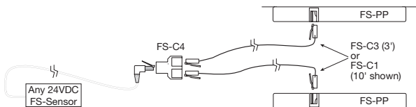
Fig 6: One sensor controlling two Power Packs
