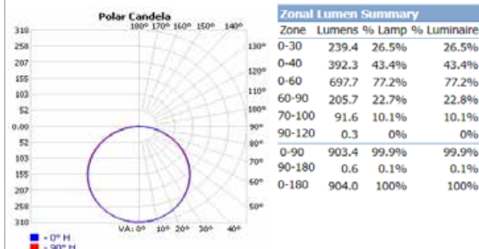
FSDLS6FR12/CCT/LED Settings: 12W at 2700K
