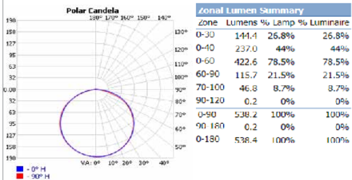
FSDLS3FR8/CCT/LED Settings: 8W at 2700K
