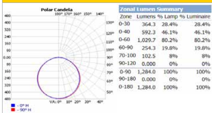
FSDLS4FR10/SQ/CCT/LED Settings: 10W at 2700K
