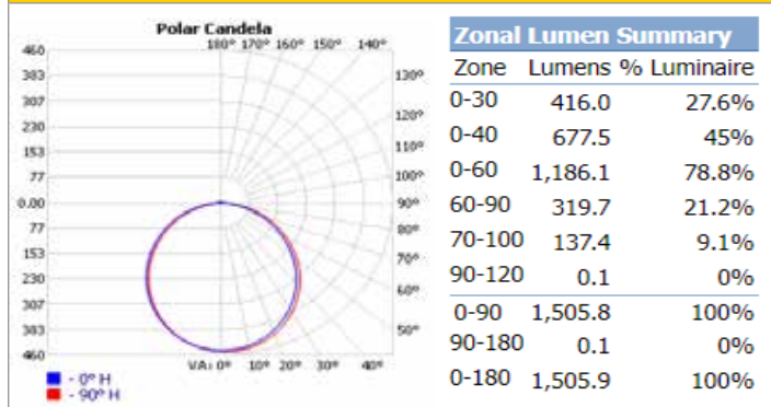
FSDLS6FR15/SQ/CCT/LED Settings: 15W at 2700K
