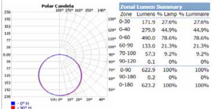
FSDLS5FR12/CCT/LED Settings: 12W at 2700K
