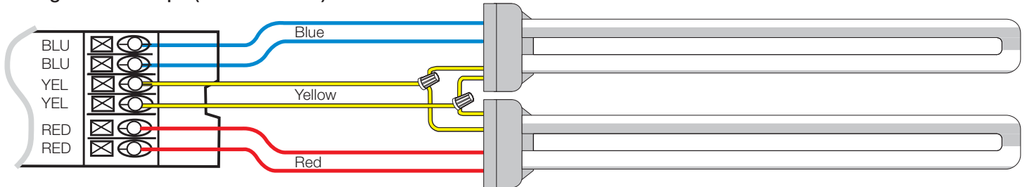
Wiring to Two Lamps (C case shown)
