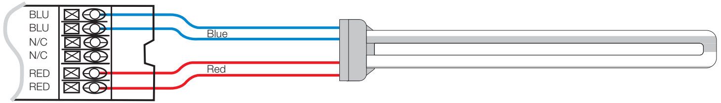
Wiring to One Lamp (C case shown)
