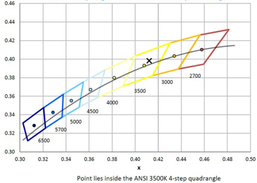
CIE 1931 Chromaticity Diagram and 2015 ANSI 7-Step Quadrangles
