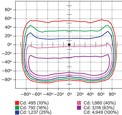
ISOCANDELA PLOT
