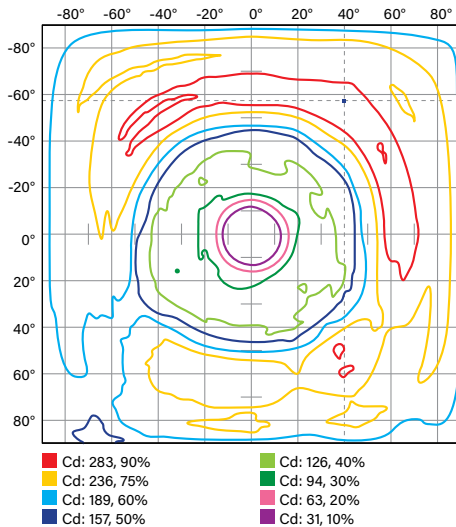
ISOCANDELA PLOT
