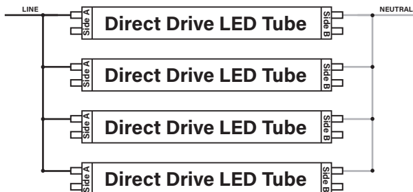
Shunted Lampholders
