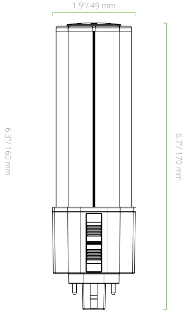
L17W GX24D BASE OMNIDIRECTIONAL
