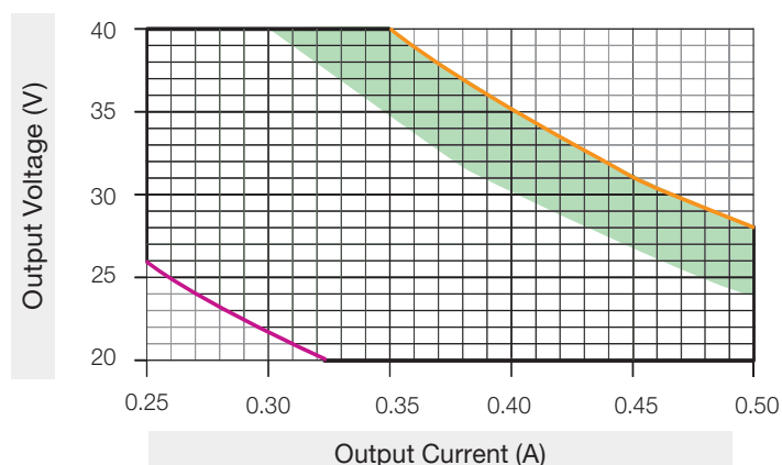
Load Compatibility
