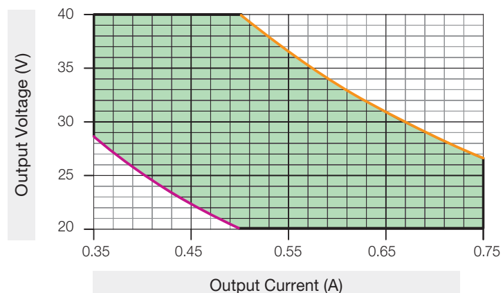
Load Compatibility
