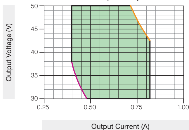
Load Compatibility
