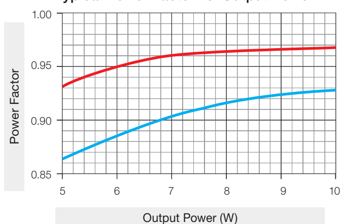
Typical Power Factor vs. Output Power
