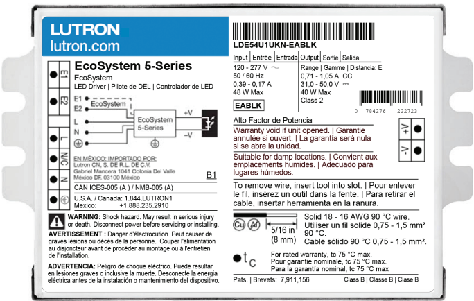
Case type K 3.00 in (76 mm) W × 1.00 in (25 mm) H × 4.90 in (124 mm) L
