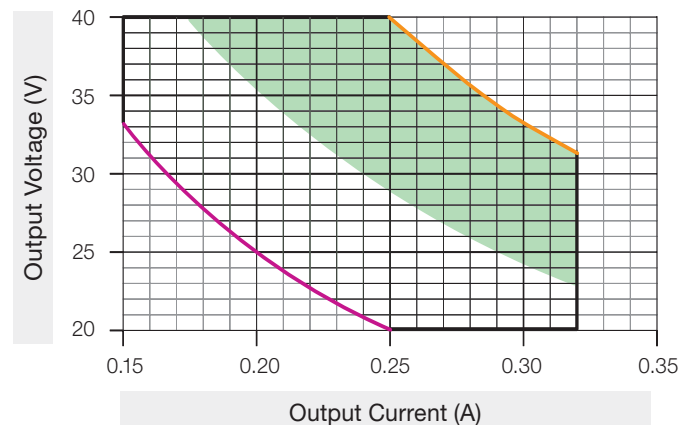
Load Compatibility
