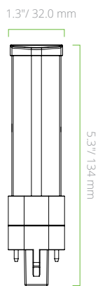
L3.5W G23 BASE HORIZONTAL
