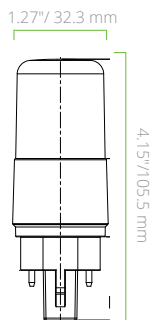
L5W G23 BASE OMNI-DIRECTIONAL
