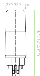
L7W GX23 BASE OMNI-DIRECTIONAL
