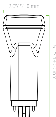
L6W G24D BASE VERTICAL
