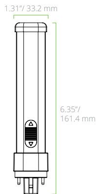
L8.5W G24D BASE HORIZONTAL (CCT SELECTABLE)
