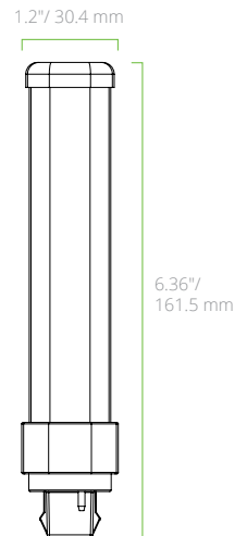
L8.5W G24D BASE HORIZONTAL
