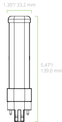
L5.5W GX23 ROTATABLE BASE HORIZONTAL
