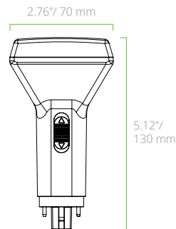
L8.5W G24D BASE VERTICAL (CCT SELECTABLE)
