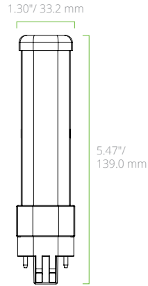
L5.5W GX23 ROTATABLE BASE HORIZONTAL
