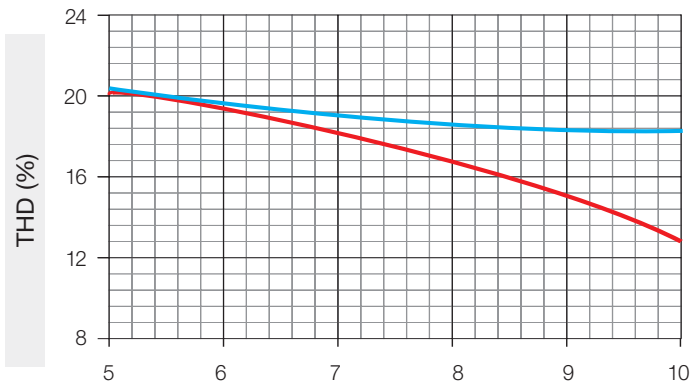
Typical THD vs. Output Power
