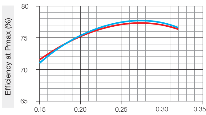
Typical Efficiency vs Output Current
