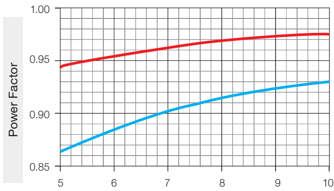
Typical Power Factor vs. Output Power
